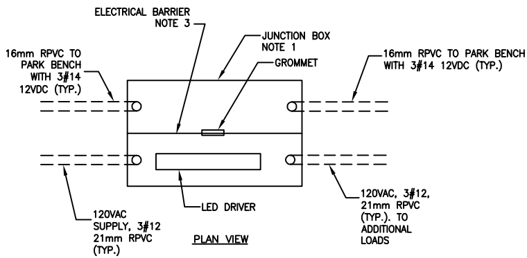
2 LED DRIVER JUNCTION BOX N.T.S.
