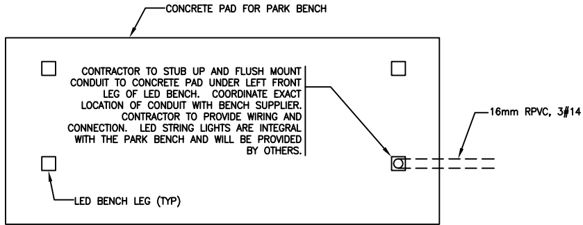
1 TYPICAL LED PARK BENCH CONNECTION – PLAN VIEW N.T.S.
