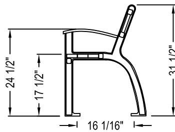
SIDE ELEVATION
