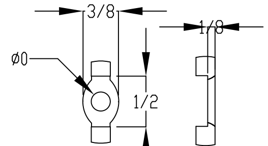
COINING DETAIL SCALE 1:1
